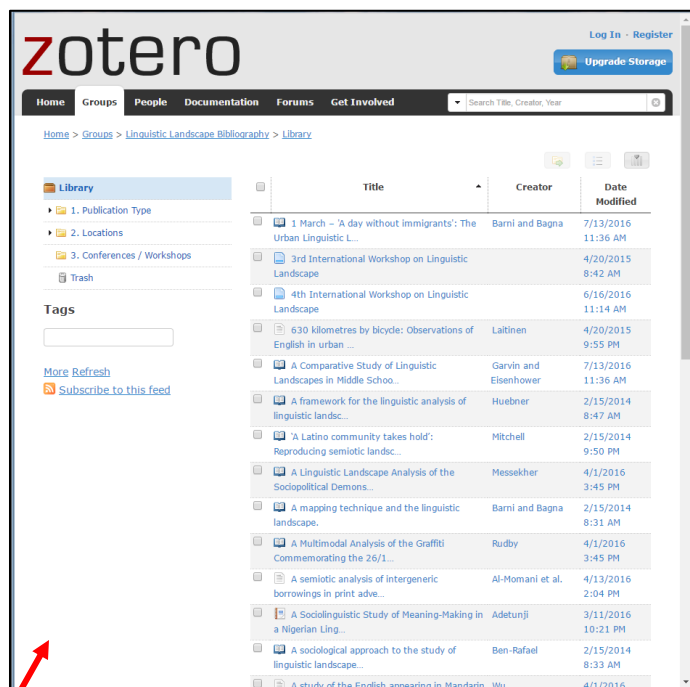
Figure 2. Group Library
